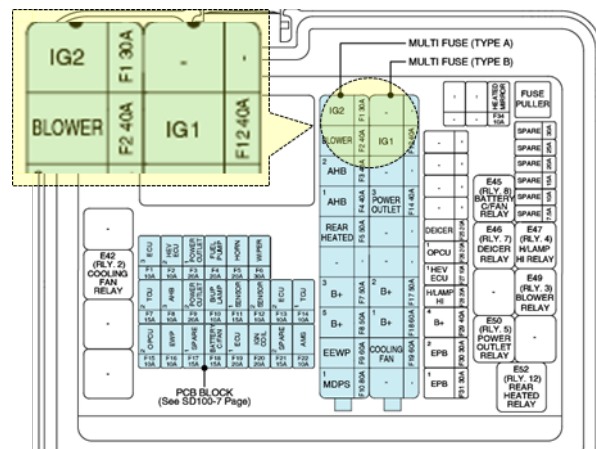
Engine room fuse box
