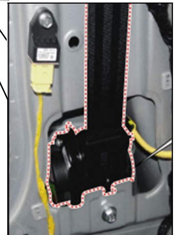
1. Front Seatbelt Pretensioner
